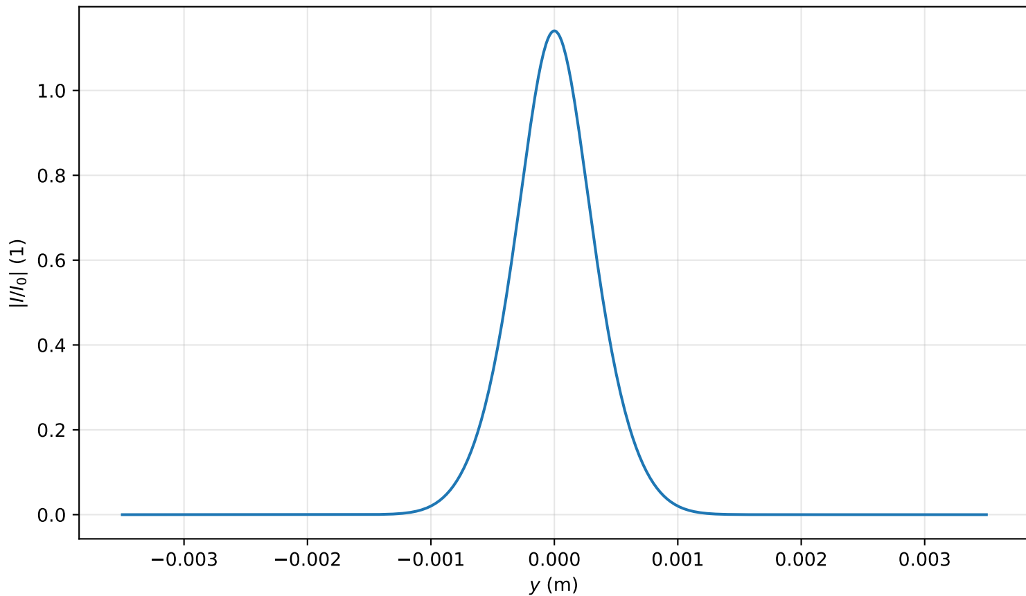
Intensity profile I(x=0, y, z=0.557)/I_0 , P_{in}=0.8P_{cr} , artificial time
